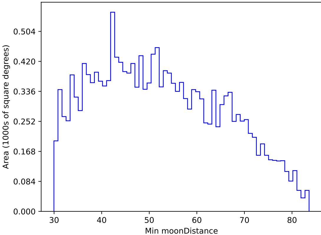
too_5_4v3.4_10yrs WFD u band: Min moonDistance
