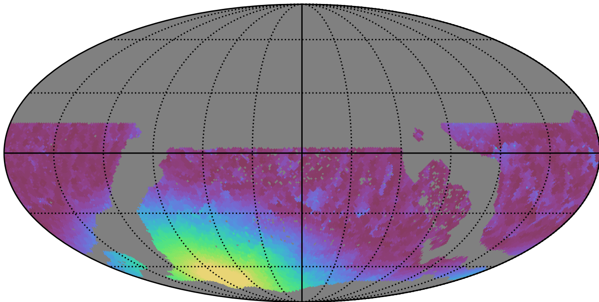
too_5_4v3.4_10yrs WFD r band: Min moonDistance
