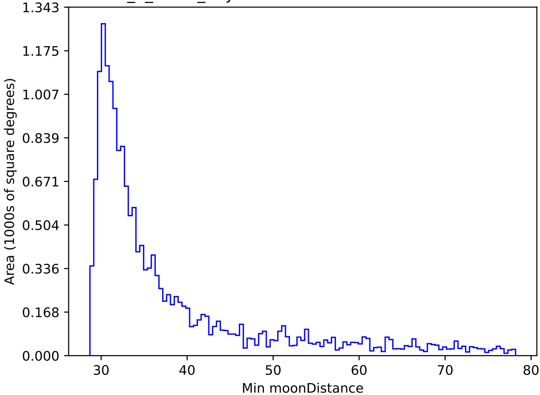
too_5_4v3.4_10yrs WFD r band: Min moonDistance
