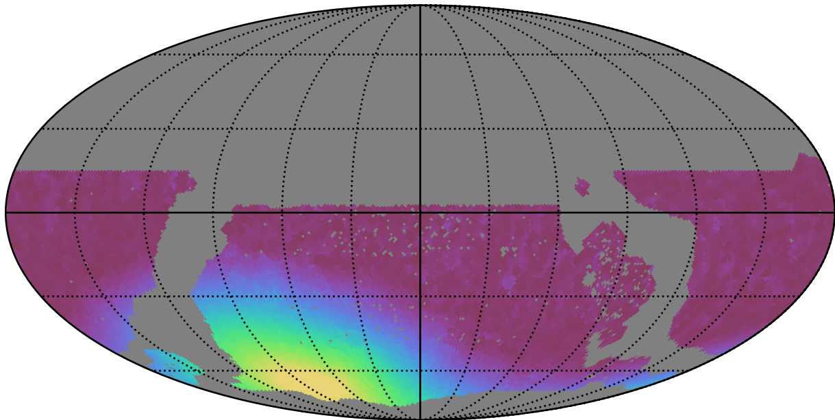
too_5_4v3.4_10yrs WFD i band: Min moonDistance
