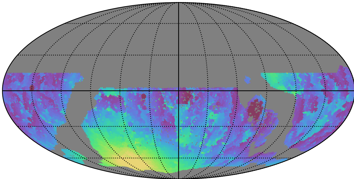
too_5_4v3.4_10yrs WFD g band: Min moonDistance
