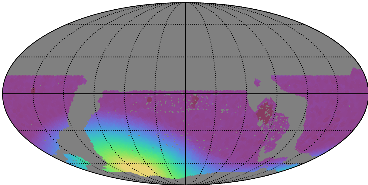
too_5_4v3.4_10yrs WFD all bands: Min moonDistance
