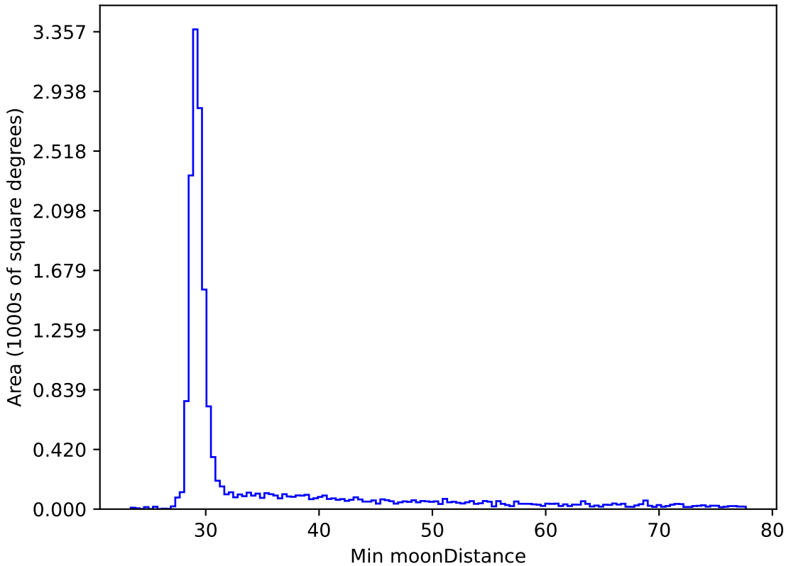
too_5_4v3.4_10yrs WFD all bands: Min moonDistance
