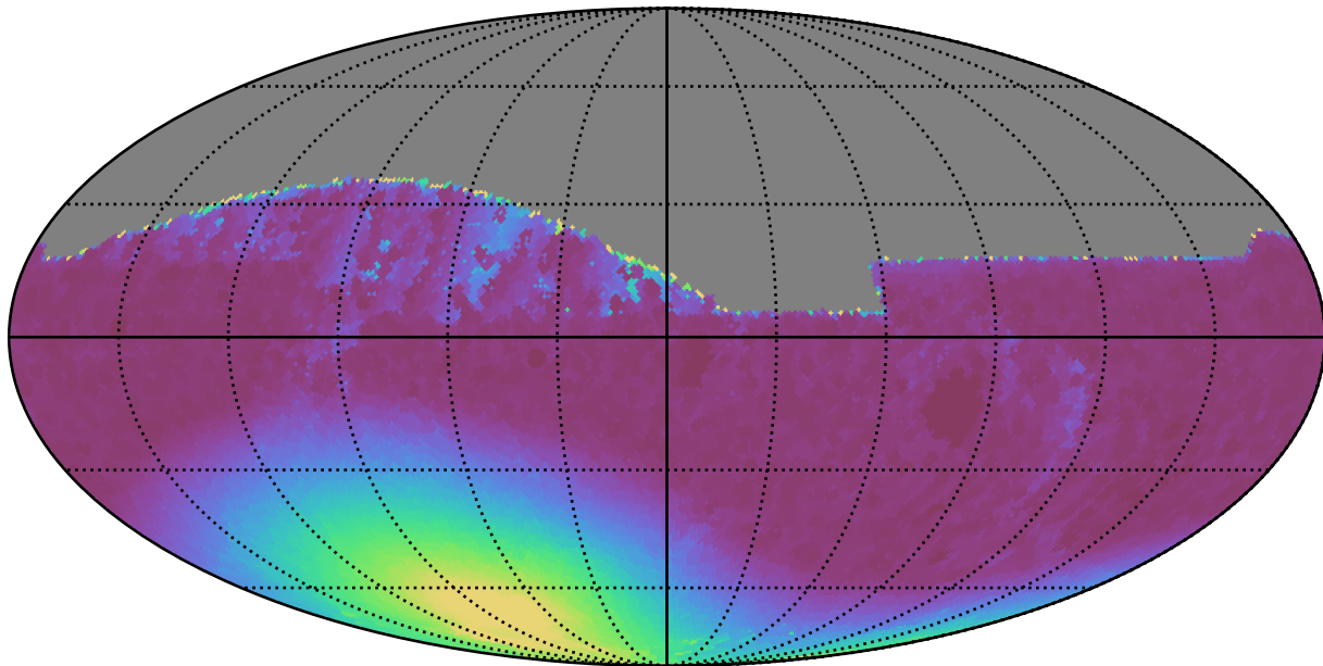
too_5_4v3.4_10yrs All sky z band: Min moonDistance
