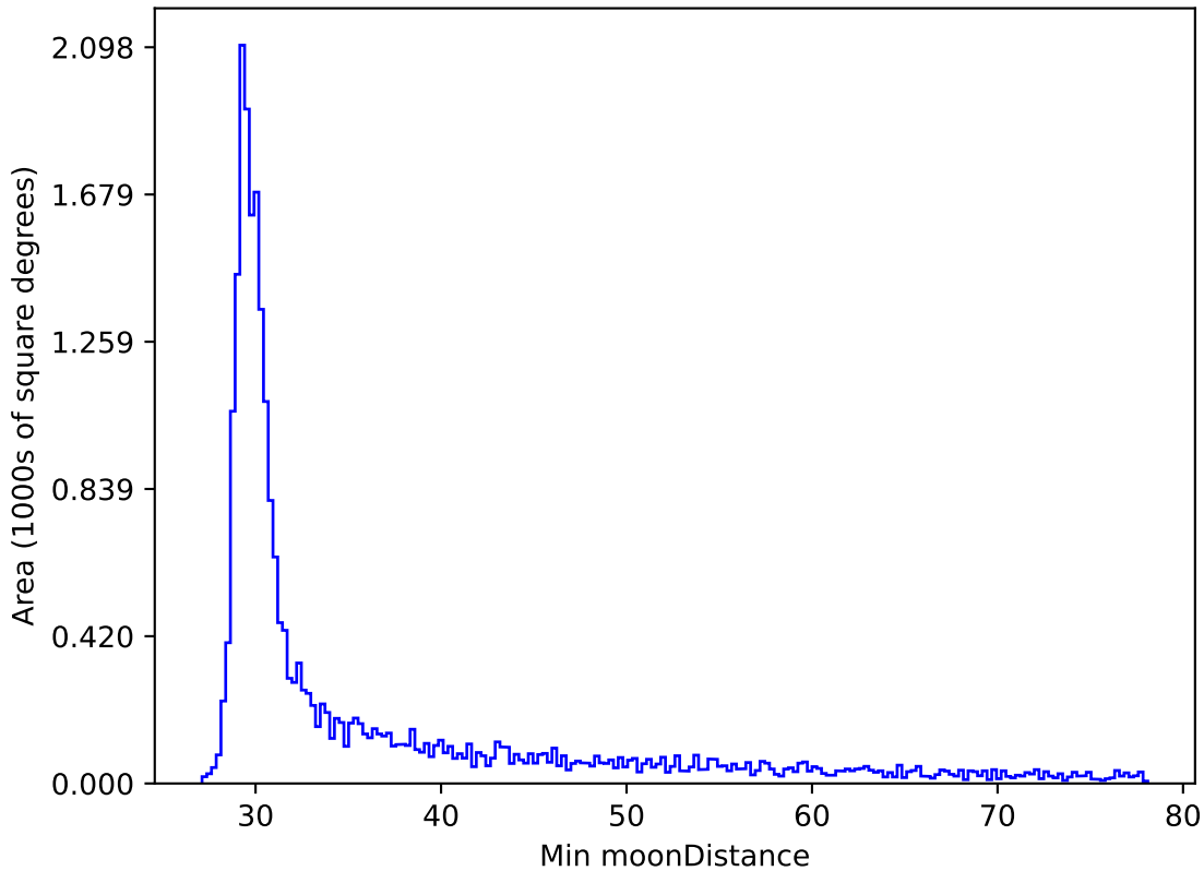
too_5_4v3.4_10yrs All sky z band: Min moonDistance
