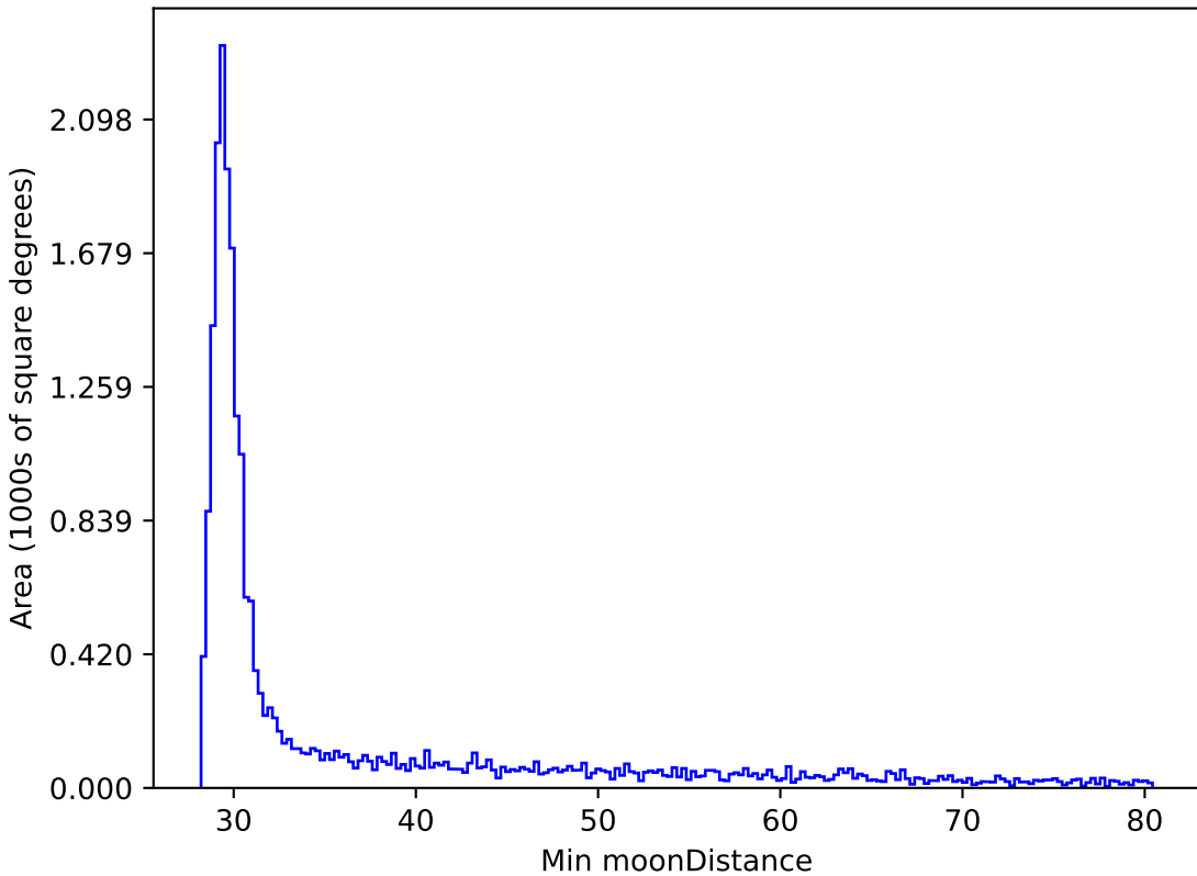
too_5_4v3.4_10yrs All sky y band: Min moonDistance
