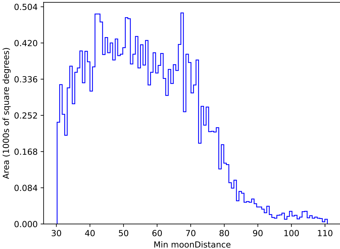
too_5_4v3.4_10yrs All sky u band: Min moonDistance
