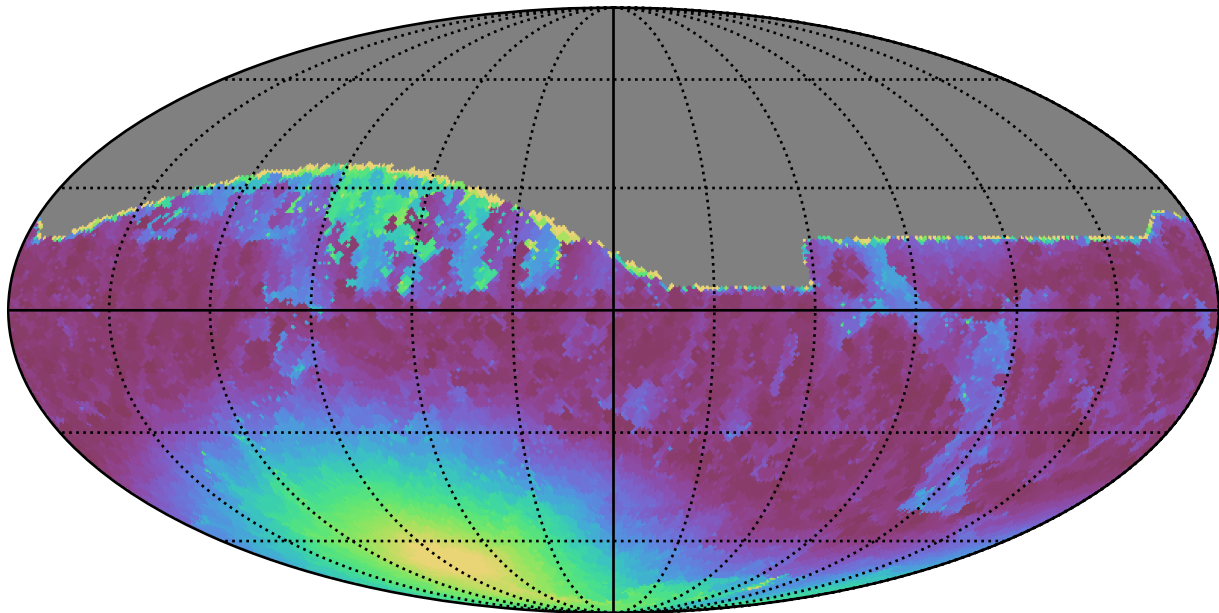
too_5_4v3.4_10yrs All sky r band: Min moonDistance
