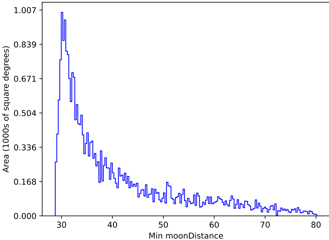
too_5_4v3.4_10yrs All sky r band: Min moonDistance
