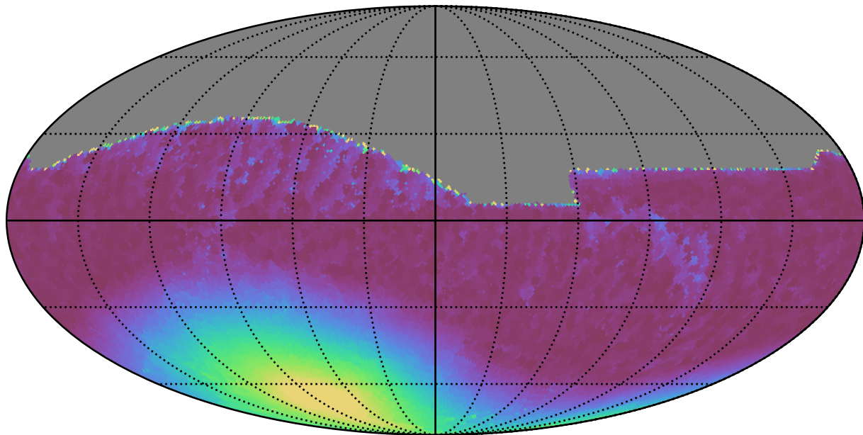
too_5_4v3.4_10yrs All sky i band: Min moonDistance
