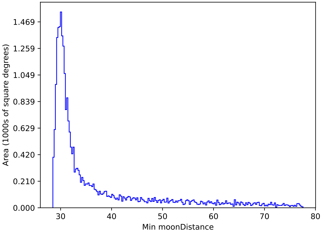
too_5_4v3.4_10yrs All sky i band: Min moonDistance
