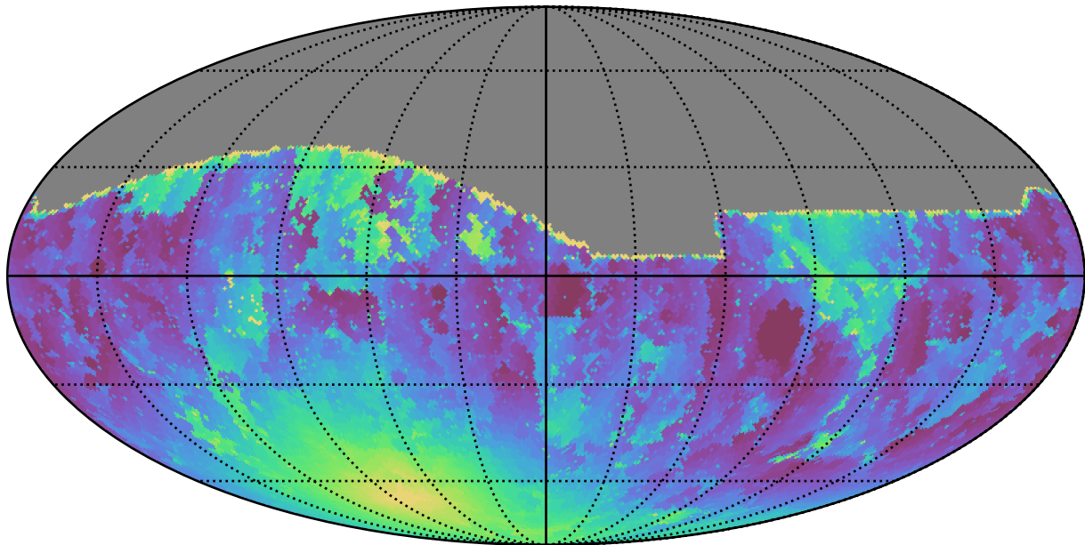
too_5_4v3.4_10yrs All sky g band: Min moonDistance
