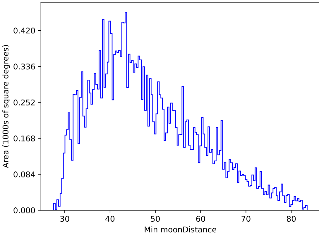
too_5_4v3.4_10yrs All sky g band: Min moonDistance
