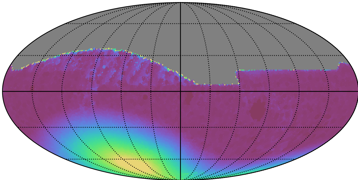
too_5_4v3.4_10yrs All sky all bands: Min moonDistance
