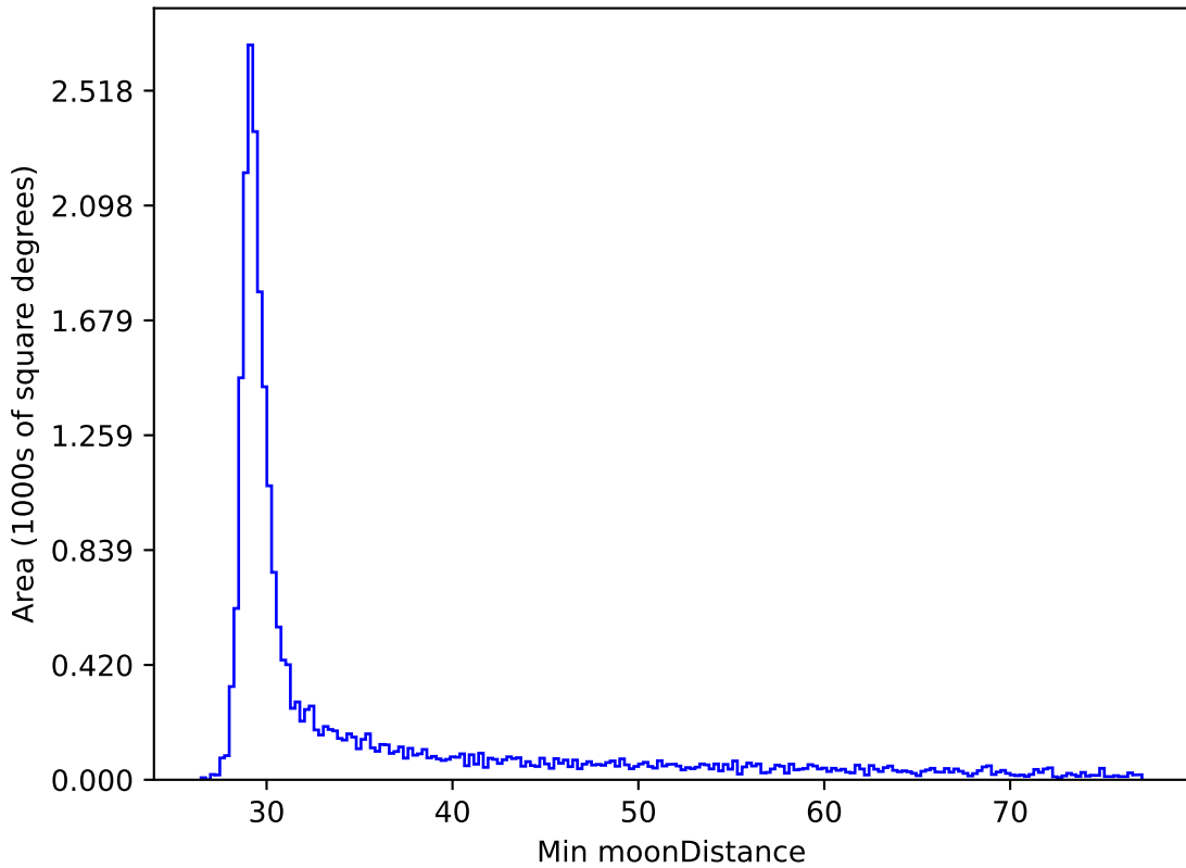
too_5_4v3.4_10yrs All sky all bands: Min moonDistance
