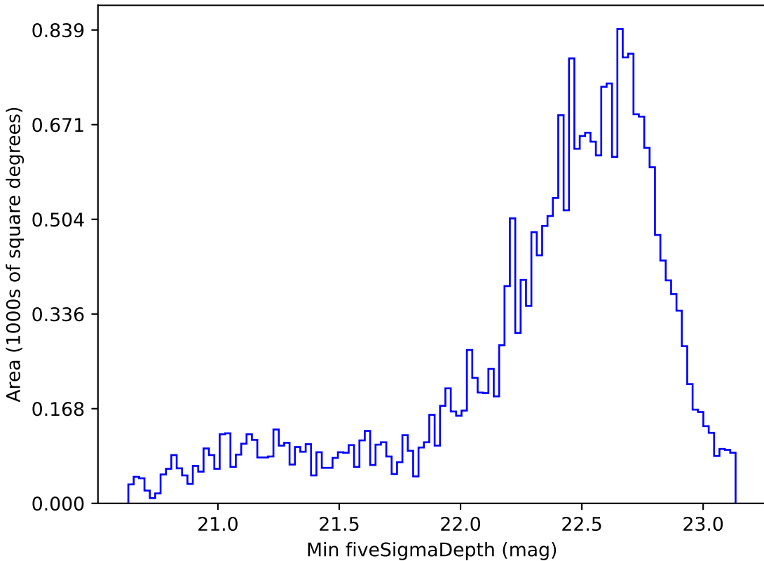
too_5_4v3.4_10yrs Yr 1 z band: Min fiveSigmaDepth
