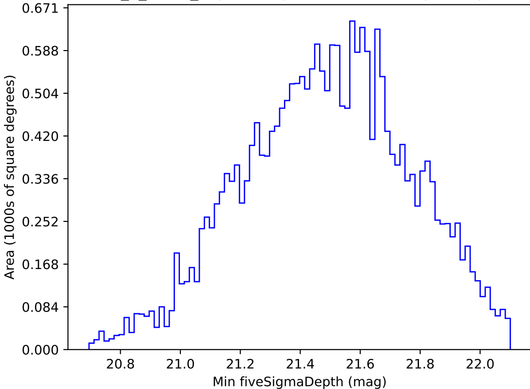
too_5_4v3.4_10yrs Yr 1 y band: Min fiveSigmaDepth
