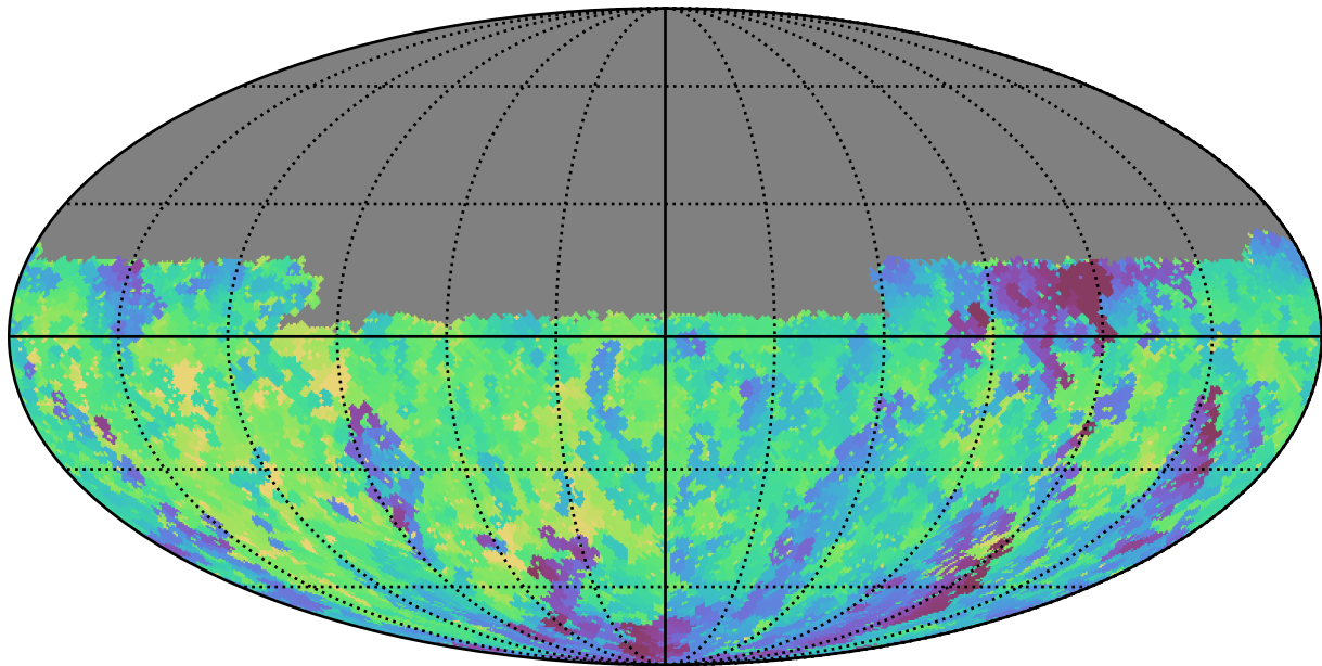
too_5_4v3.4_10yrs Yr 1 u band: Min fiveSigmaDepth
