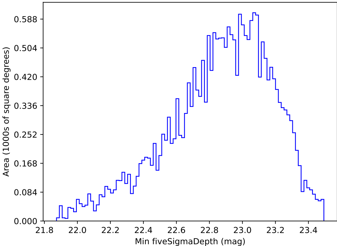
too_5_4v3.4_10yrs Yr 1 u band: Min fiveSigmaDepth
