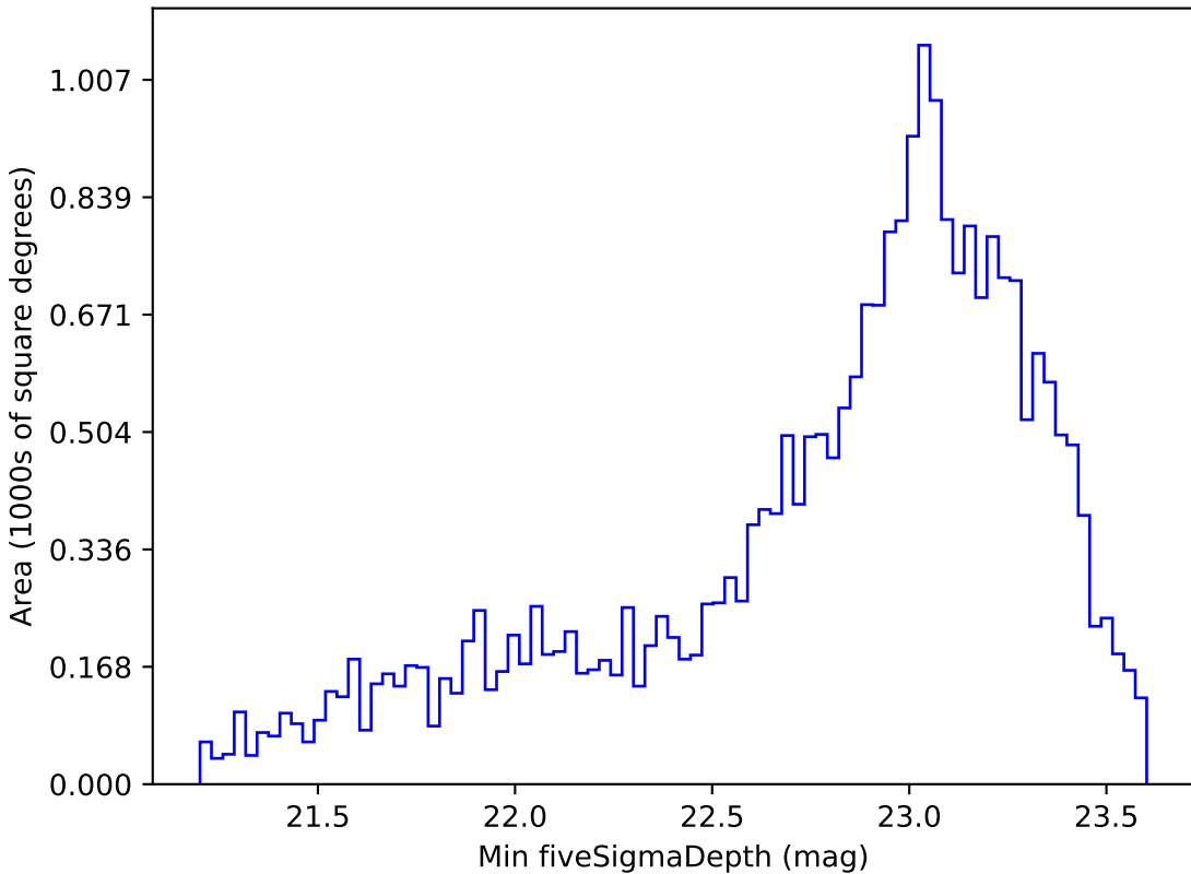
too_5_4v3.4_10yrs Yr 1 i band: Min fiveSigmaDepth
