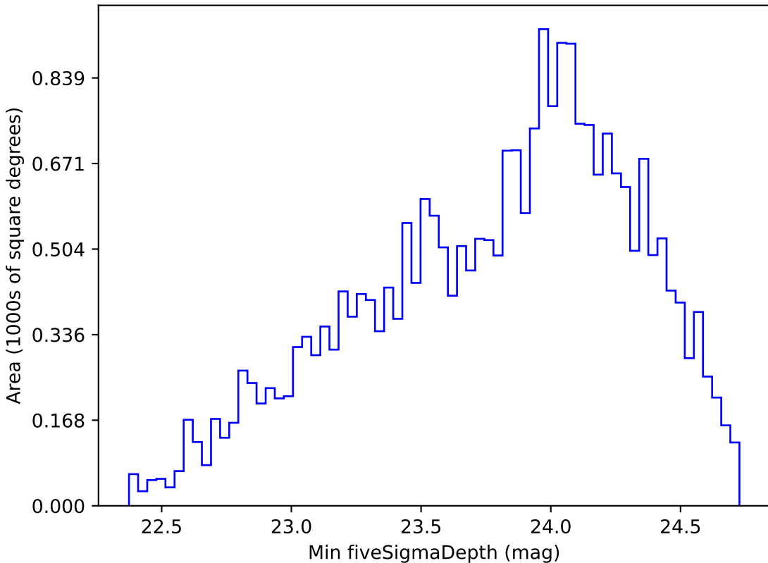
too_5_4v3.4_10yrs Yr 1 g band: Min fiveSigmaDepth
