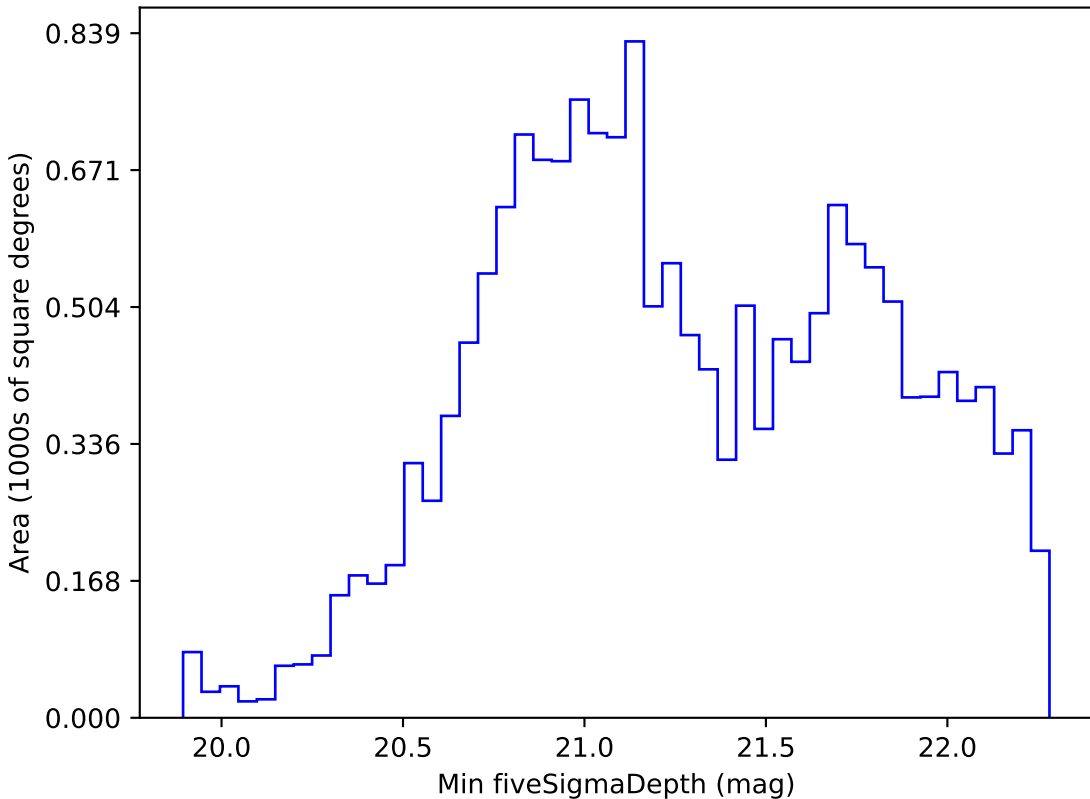
too_5_4v3.4_10yrs WFD z band: Min fiveSigmaDepth
