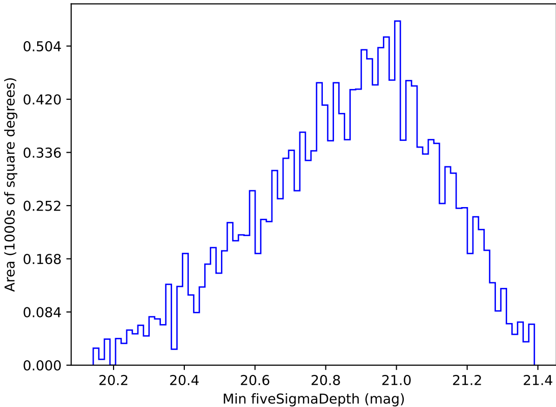
too_5_4v3.4_10yrs WFD y band: Min fiveSigmaDepth
