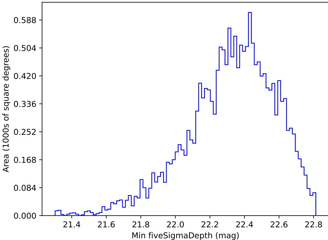
too_5_4v3.4_10yrs WFD u band: Min fiveSigmaDepth
