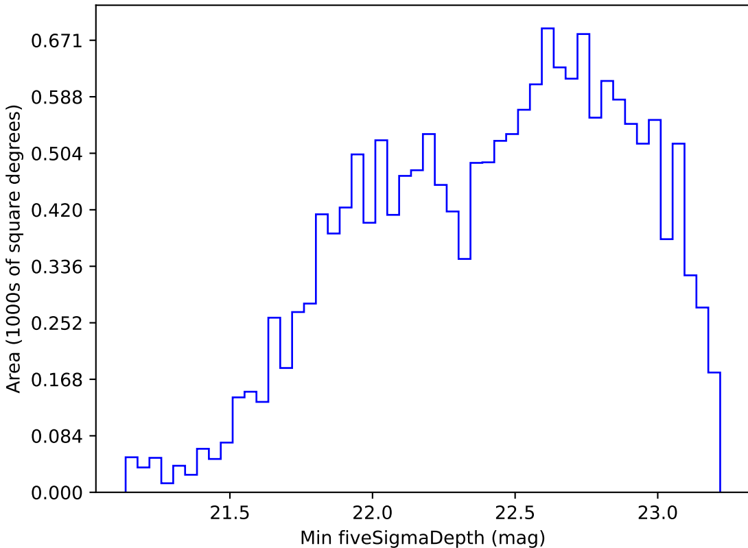
too_5_4v3.4_10yrs WFD r band: Min fiveSigmaDepth
