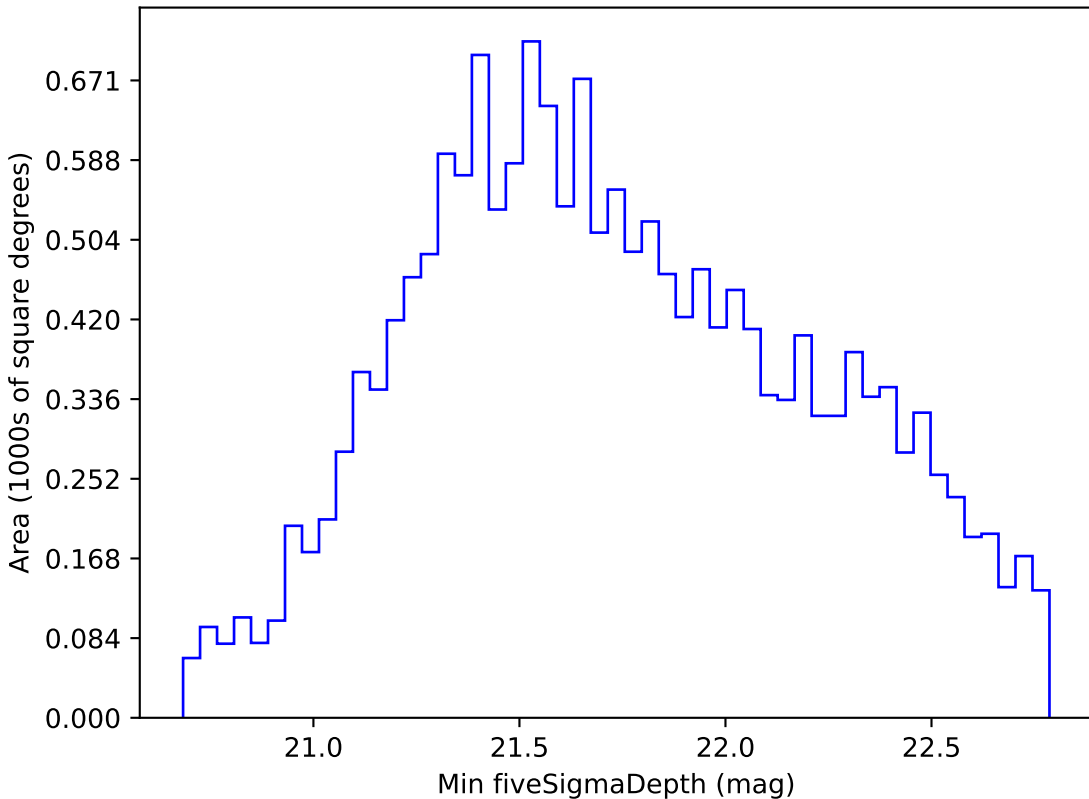
too_5_4v3.4_10yrs WFD i band: Min fiveSigmaDepth
