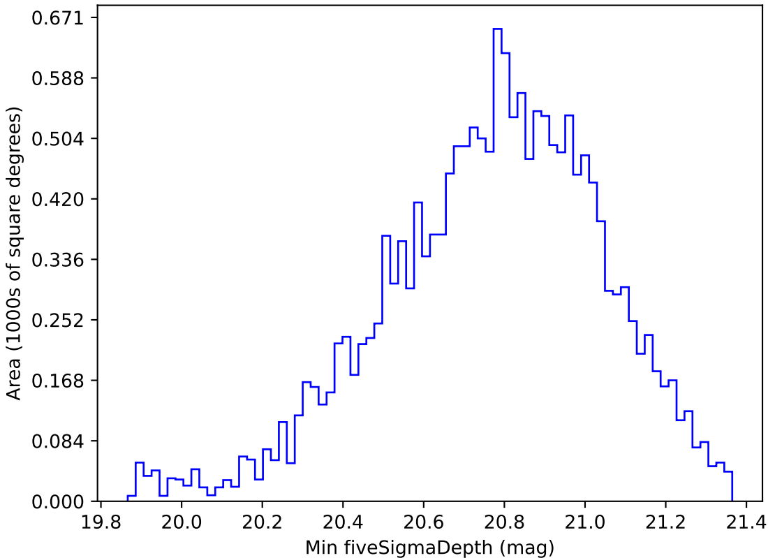
too_5_4v3.4_10yrs WFD all bands: Min fiveSigmaDepth
