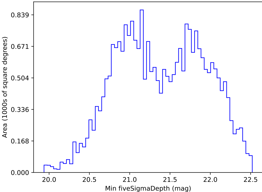
too_5_4v3.4_10yrs All sky z band: Min fiveSigmaDepth
