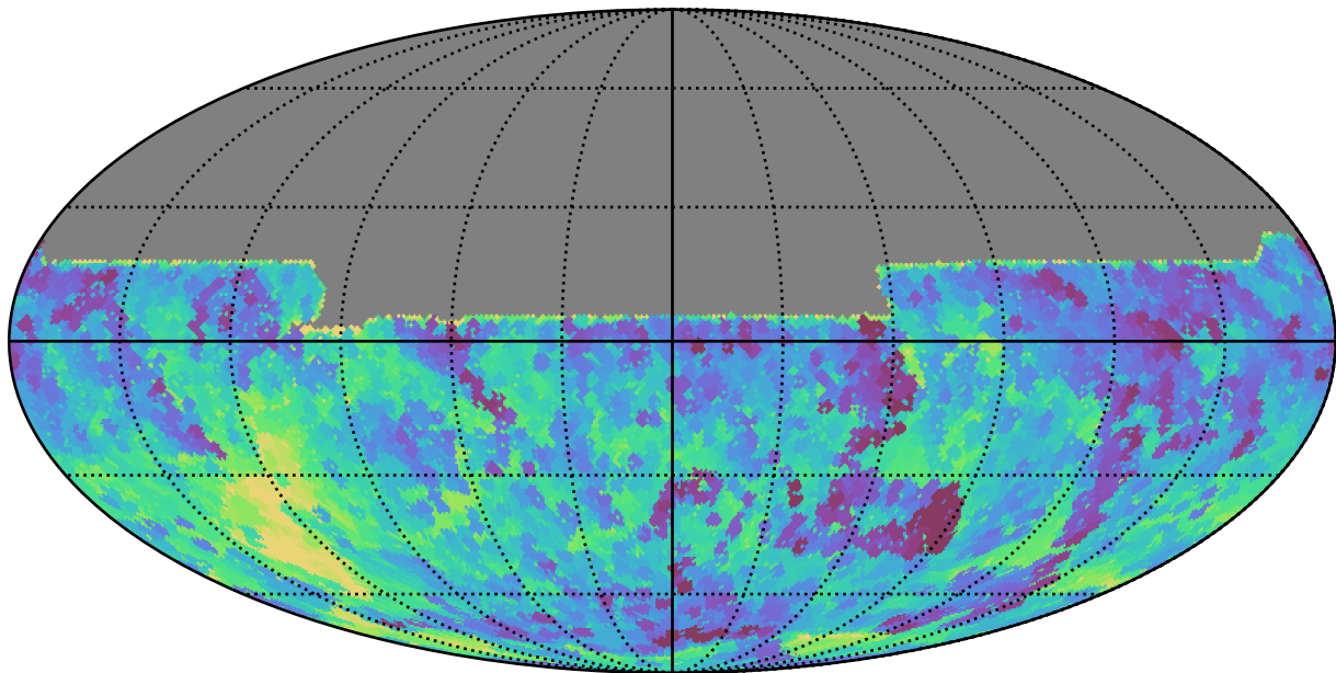
too_5_4v3.4_10yrs All sky y band: Min fiveSigmaDepth
