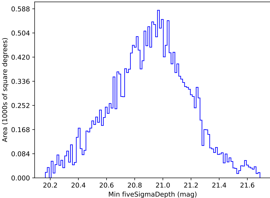
too_5_4v3.4_10yrs All sky y band: Min fiveSigmaDepth
