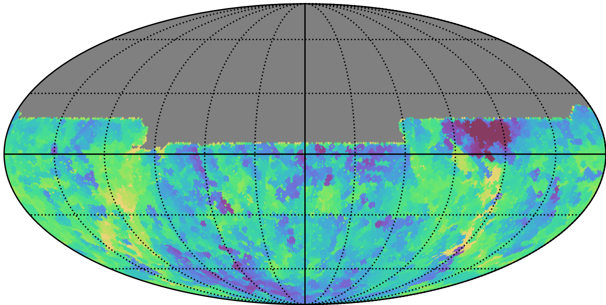
too_5_4v3.4_10yrs All sky u band: Min fiveSigmaDepth
