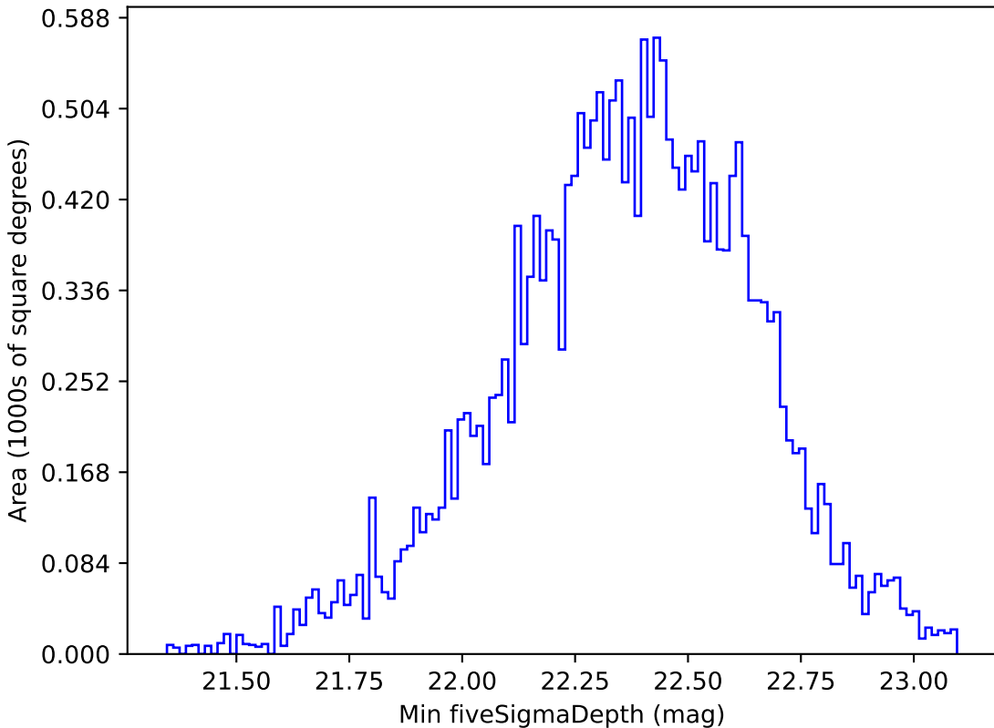
too_5_4v3.4_10yrs All sky u band: Min fiveSigmaDepth
