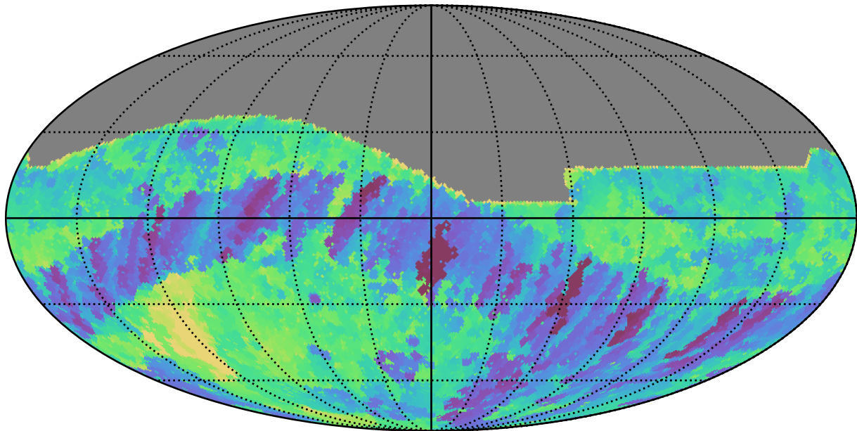
too_5_4v3.4_10yrs All sky r band: Min fiveSigmaDepth
