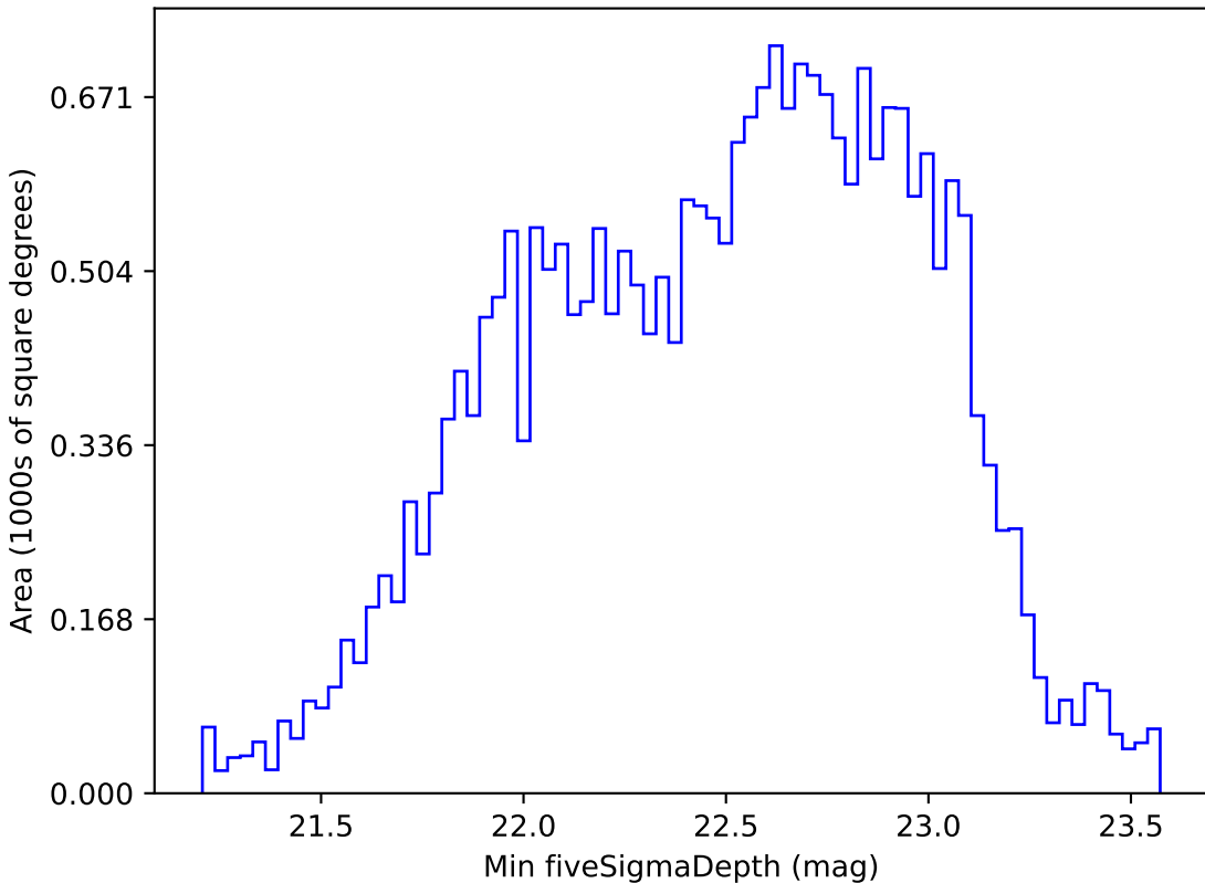
too_5_4v3.4_10yrs All sky r band: Min fiveSigmaDepth
