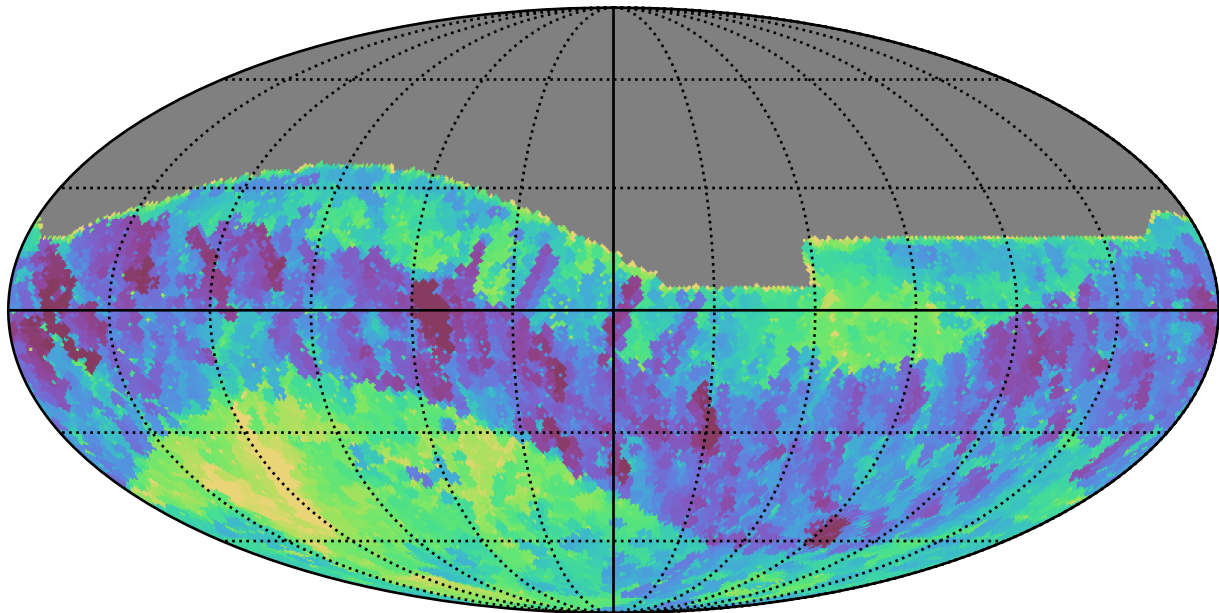
too_5_4v3.4_10yrs All sky i band: Min fiveSigmaDepth
