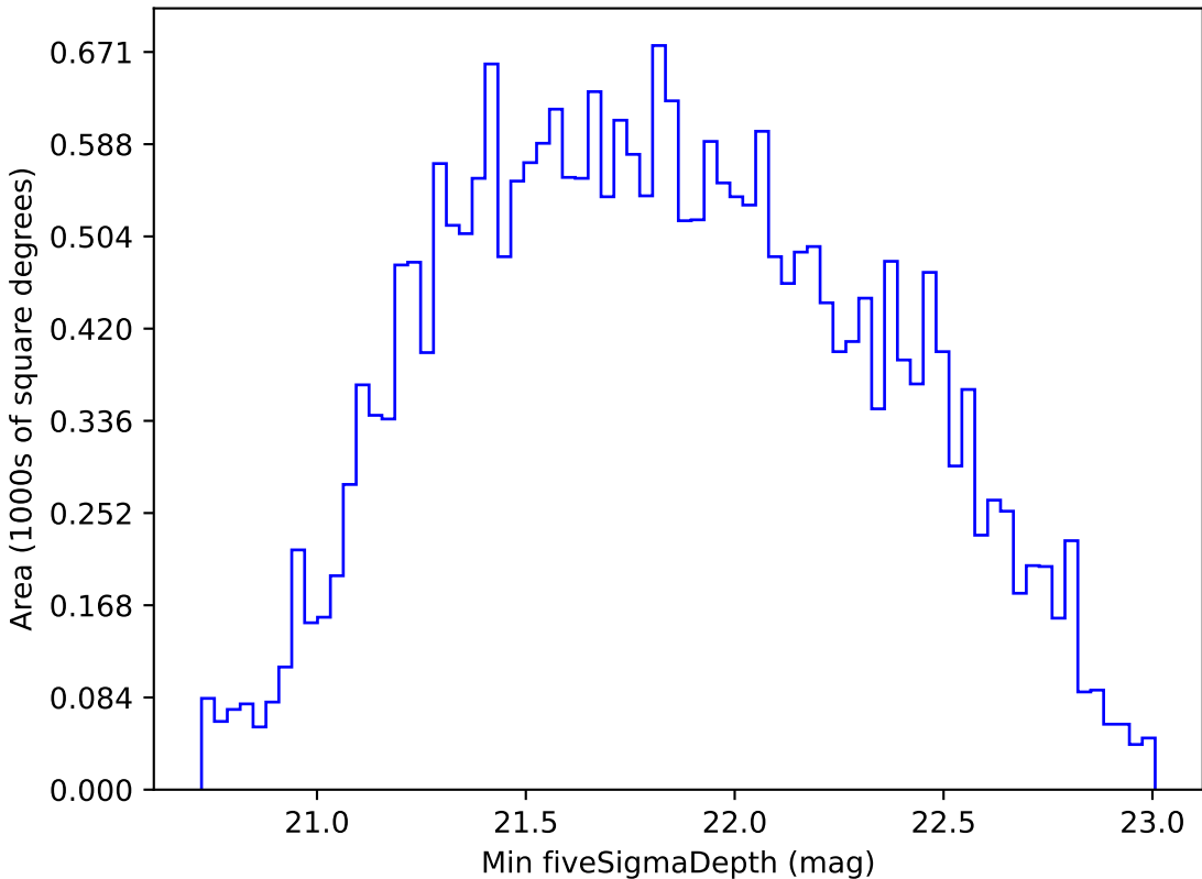
too_5_4v3.4_10yrs All sky i band: Min fiveSigmaDepth
