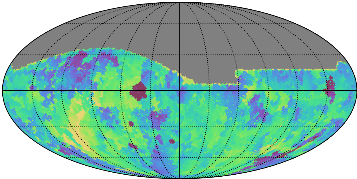
too_5_4v3.4_10yrs All sky g band: Min fiveSigmaDepth
