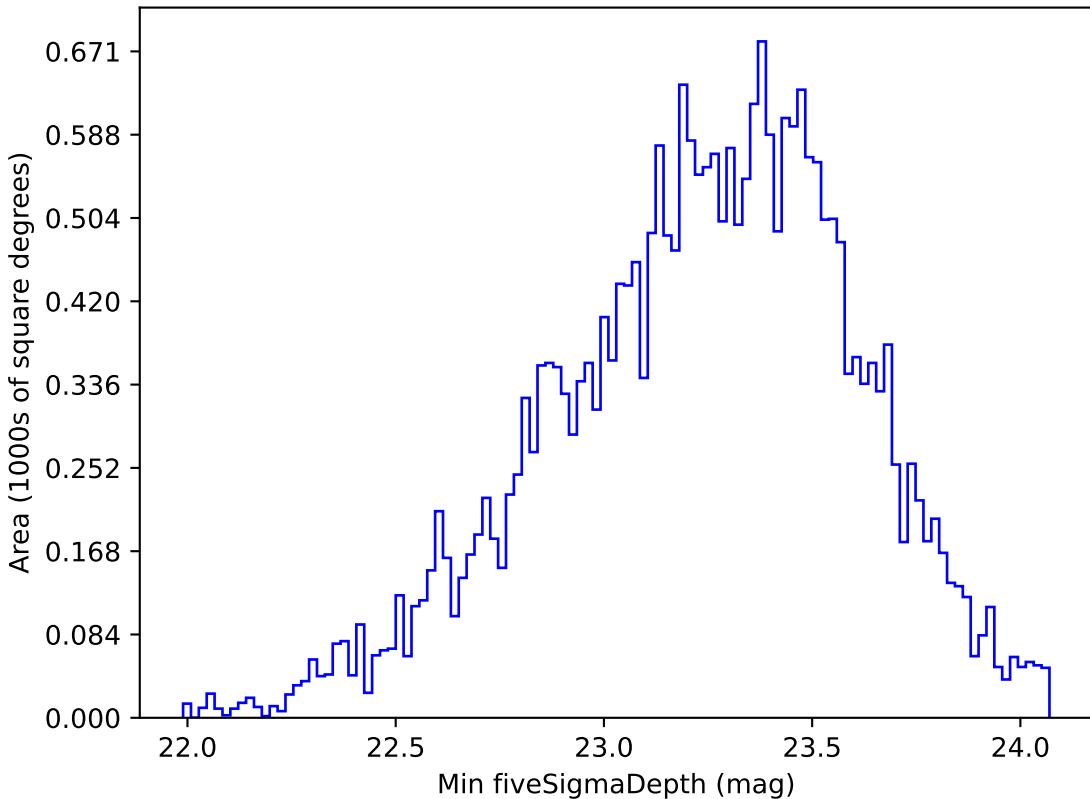
too_5_4v3.4_10yrs All sky g band: Min fiveSigmaDepth
