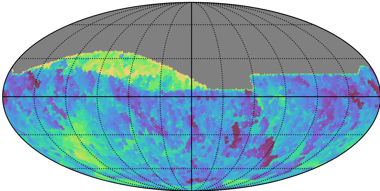
too_5_4v3.4_10yrs All sky all bands: Min fiveSigmaDepth
