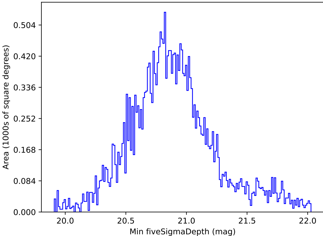
too_5_4v3.4_10yrs All sky all bands: Min fiveSigmaDepth
