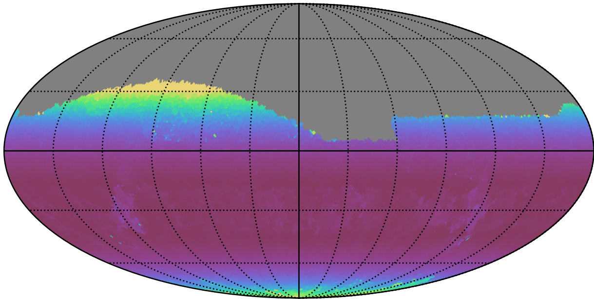
too_5_4v3.4_10yrs Yr 1 z band: Min airmass
