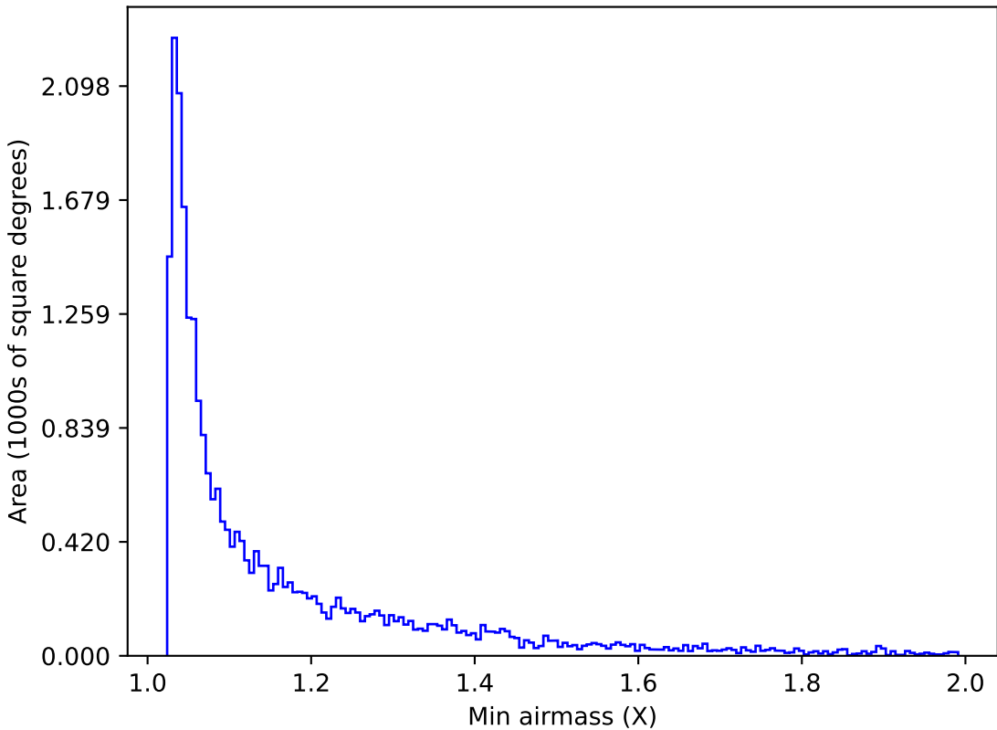
too_5_4v3.4_10yrs Yr 1 z band: Min airmass
