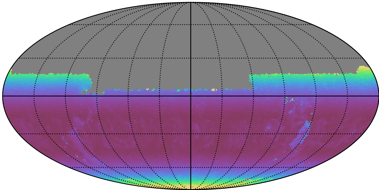
too_5_4v3.4_10yrs Yr 1 y band: Min airmass
