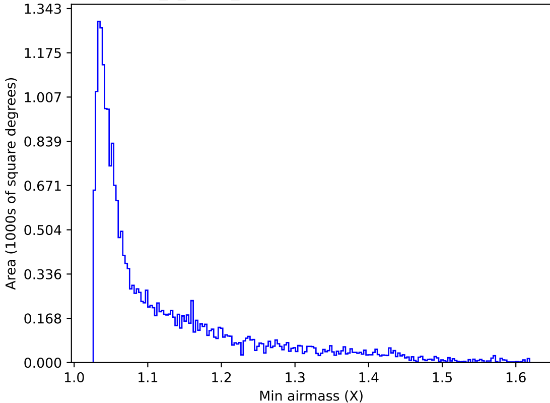
too_5_4v3.4_10yrs Yr 1 y band: Min airmass
