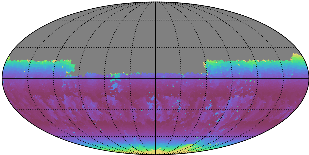
too_5_4v3.4_10yrs Yr 1 u band: Min airmass
