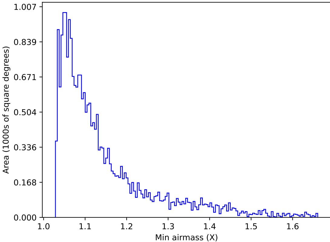
too_5_4v3.4_10yrs Yr 1 u band: Min airmass
